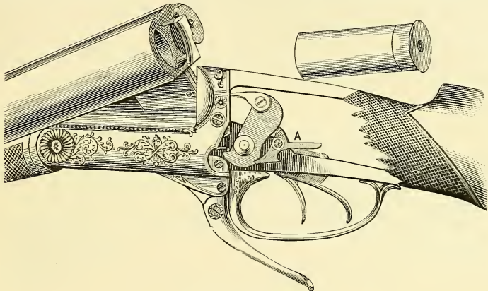
The Needham Ejector Gun.
